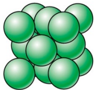
Face-centered cubic
