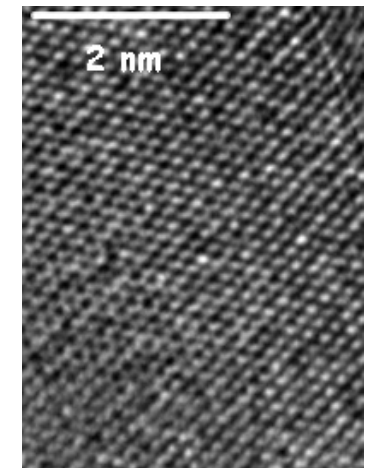
Atomes (0.1 nm)
